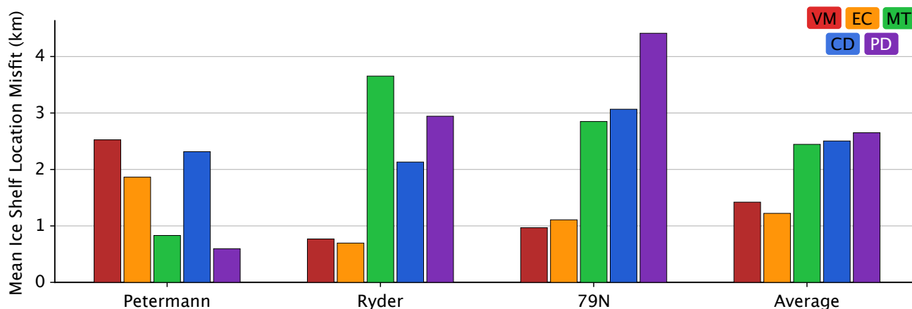
Figure 5. Misfit between modelled and observed shelf locations at the end of the calibration simulations for each calving law using tuning values that provide the best fit to terminus observations in 2024 (Table 2).
