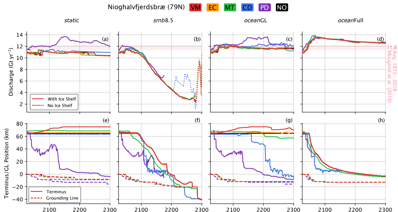
Figure 9. Model results for transient simulations of 79N to 2300 across different calving laws; VM (red), EC (orange), MT (green), CD (blue), PD (purple) and a simulation with calving turned off (NO, black). (a-d) Annual discharge rates, the transition from a solid to dotted line represents the collapse of the ice tongue to grounded calving front. (e-h) Changes in terminus (solid) and grounding line (dashed) positions with respect to their observed positions at 79N in 2024 along a central flowline.
