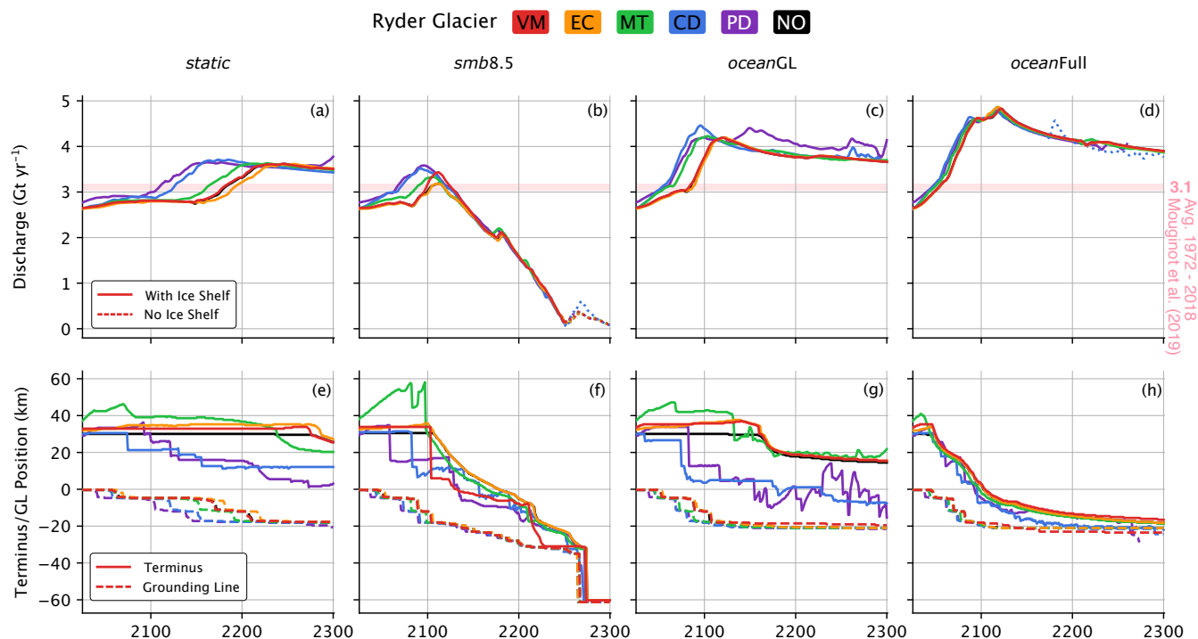
Figure 8. Model results for transient simulations of Ryder Glacier to 2300 across different calving laws; VM (red), EC (orange), MT (green), CD (blue), PD (purple) and a simulation with calving turned off (NO, black). (a-d) Annual discharge rates, the transition from a solid to dotted line represents the collapse of the ice tongue to grounded calving front. (e-h) Changes in terminus (solid) and grounding line (dashed) positions with respect to their observed positions at Ryder Glacier in 2024 along a central flowline.
