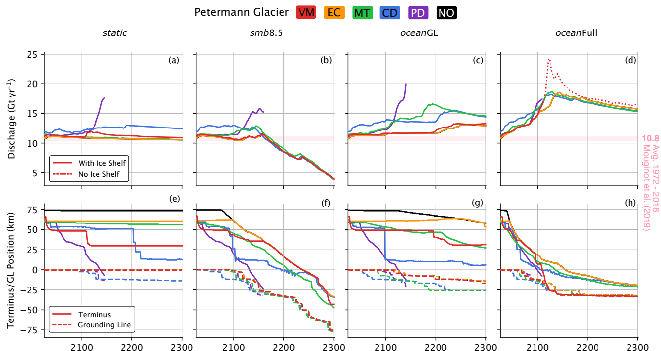
Figure 7. Model results for transient simulations of Petermann Glacier to 2300 across different calving laws; VM (red), EC (orange), MT (green), CD (blue), PD (purple) and a simulation with calving turned off (NO, black). (a-d) Annual discharge rates, the transition from a solid to dotted line represents the collapse of the ice tongue to grounded calving front. (e-h) Changes in terminus (solid) and grounding line (dashed) positions with respect to their observed positions at Petermann Glacier in 2024 along a central flowline.
