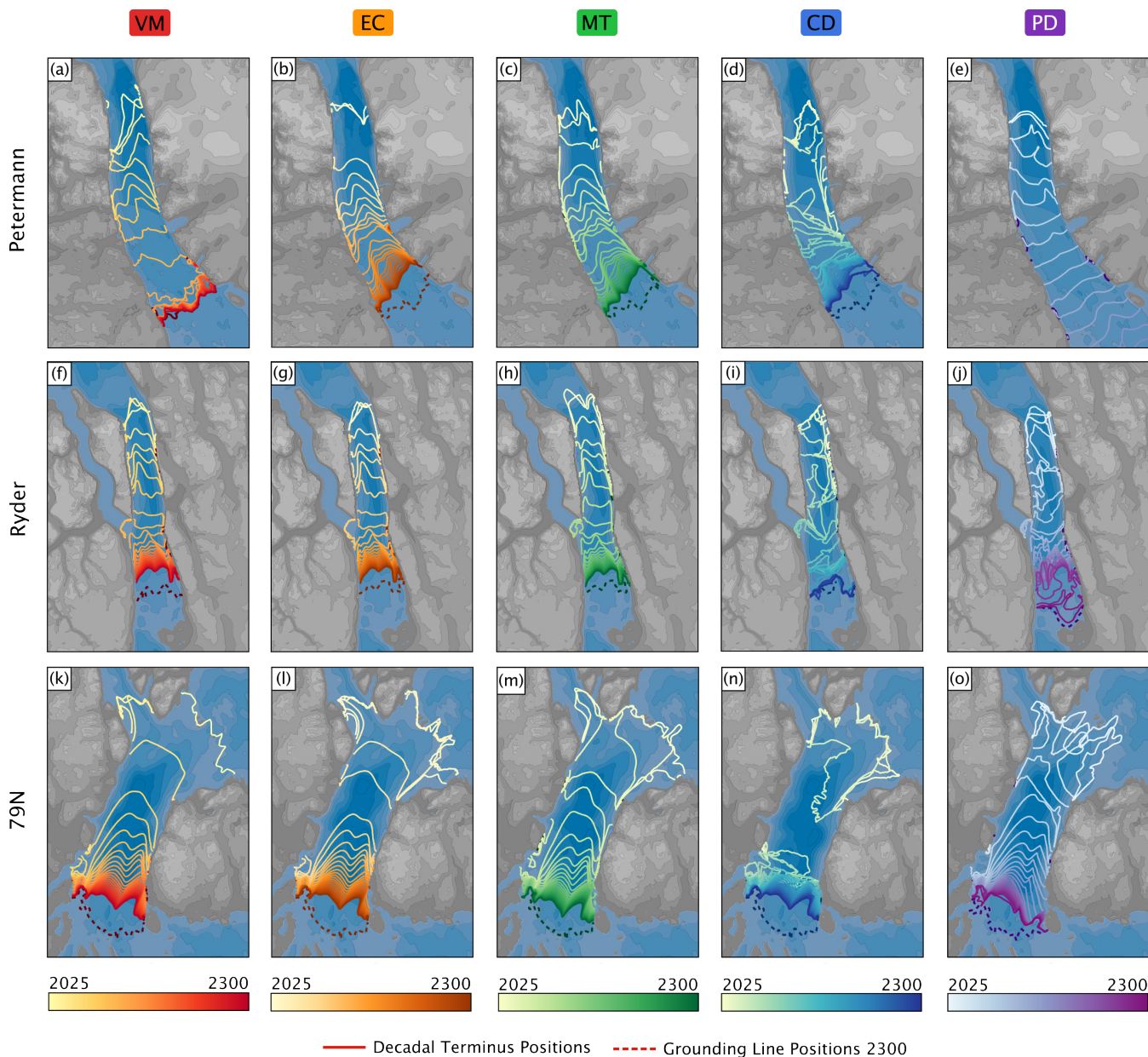
Figure 6. Evolution of the three remaining Greenlandic floating ice shelves from 2025 to 2300 under the oceanFull scenario using the five different calving laws. Terminus positions at the end of every 10 years, and including 2300, are shown with solid lines while the grounding line position in 2300 is shown with a dashed line.
