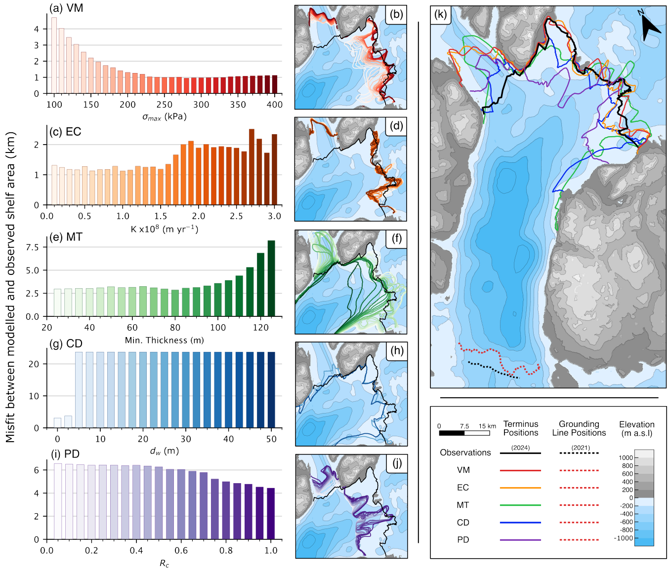
Figure 4. Calving calibrations for 79N. (a-b) Results from the Von Mises calving law: (a) showing the quantitative misfit between the observed ice shelf area in 2024 against that produced by varying the law’s tuning parameter and (b) final terminus positions of the various tuning runs against the 2024 terminus in black. Equivalent results for calving laws EC (c-d), MT (e-f) and CD (g-h) and PD (i-j). Only two modelled fronts are shown in panel h, owing to exaggerated retreat from d_w values greater than 2.5 m. i-j use \dot{M}_{max} = 2 \text{ km yr}^{-1} for the PD law, other values of \dot{M}_{max} shown in Fig. S1. (k) Comparison of final terminus and grounding line positions for the chosen best-fit calibration values (Table 2) as well as the 2024 terminus position and 2021 grounding line (Millan et al., 2023). Note that grounding line positions are consistent across all calving laws.
